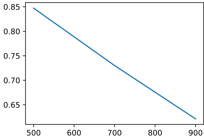
FWHM(\lambda)
