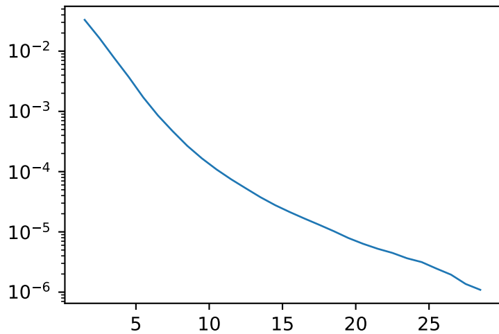
radial profile
