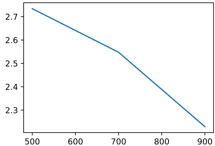
\beta(\lambda)
